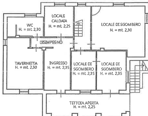
PIANO TERRA
